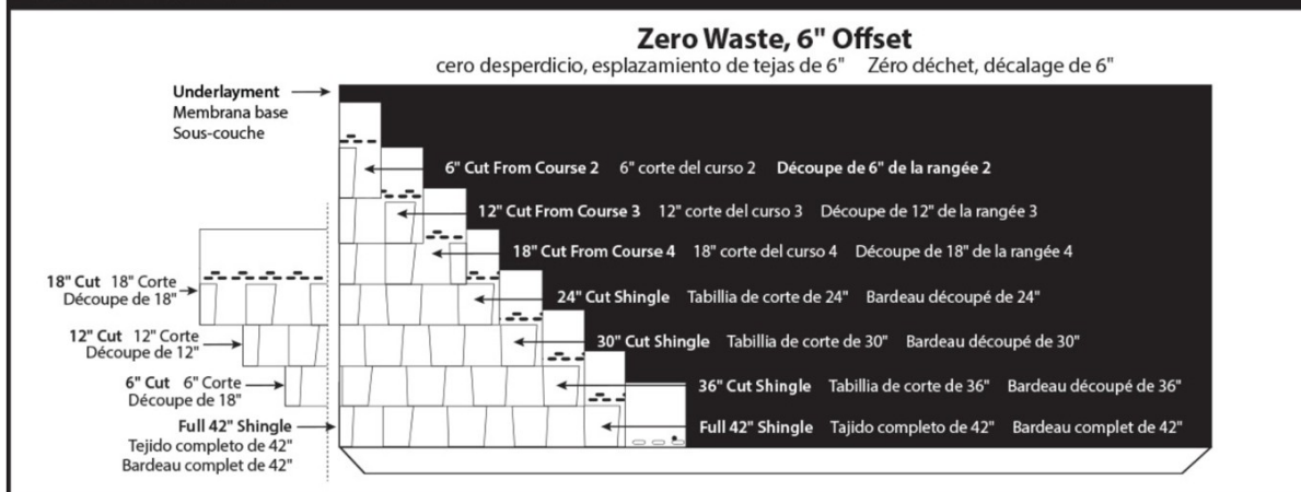
DIAGRAM 3 SHINGLE OFFSET
